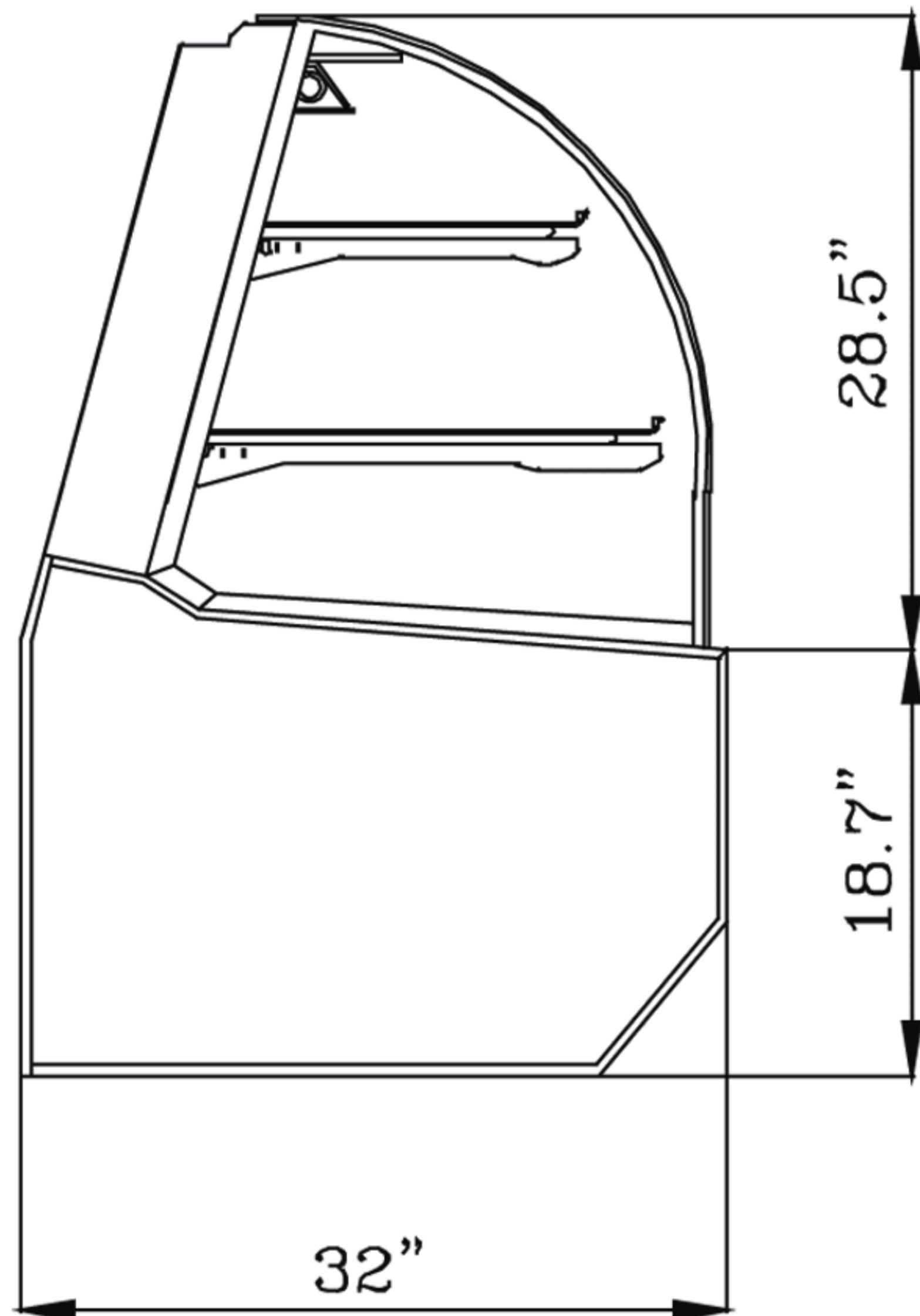
SIDE VIEW
